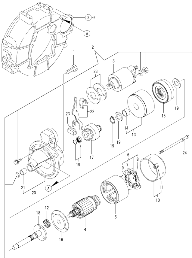
OCD10-M82001 ENGINE SECTION Fig.14. STARTING MOTOR
