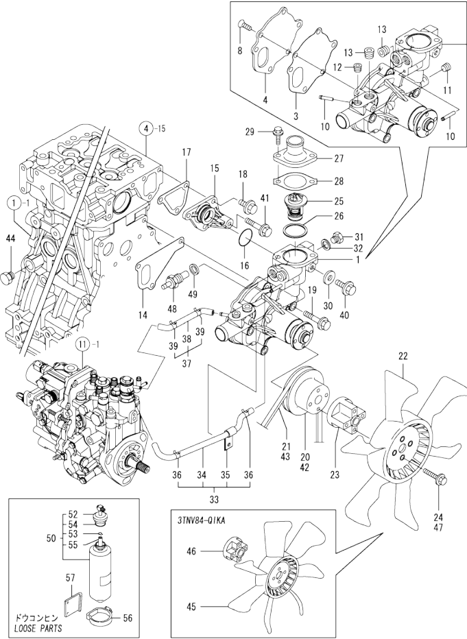
OCD10-M82001 ENGINE SECTION Fig.10. COOLING WATER SYSTEM
