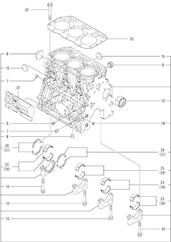
OCD10-M82001 ENGINE SECTION Fig.1. CYLINDER BLOCK
