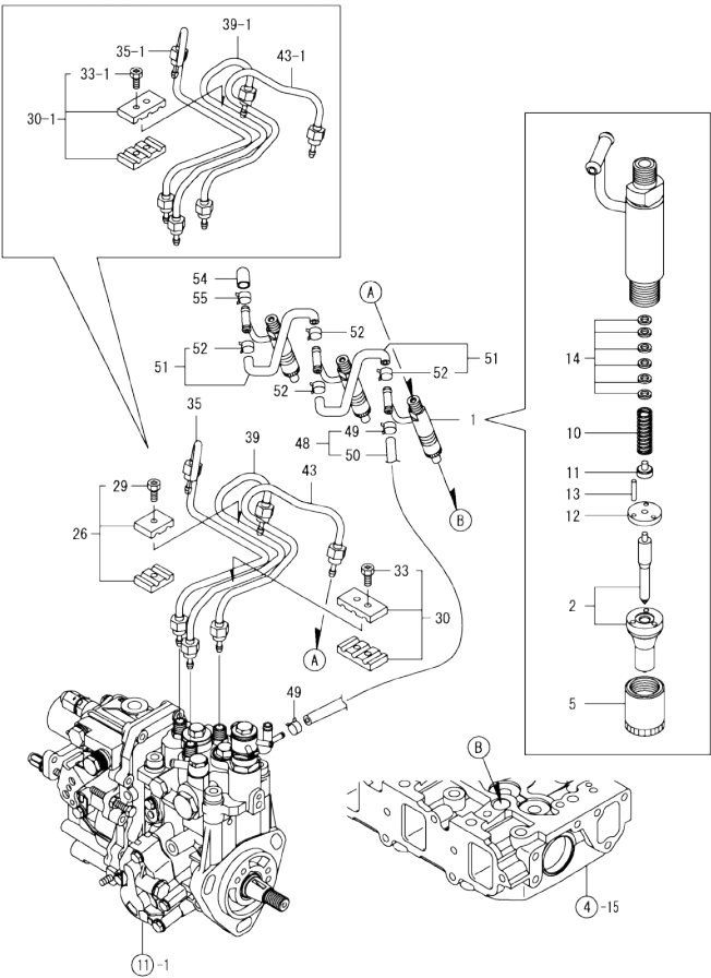
OCD10-M82001 ENGINE SECTION Fig.12. FUEL INJECTION VALVE
