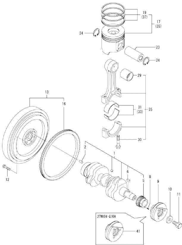
OCD10-M82001 ENGINE SECTION Fig.8. CRANKSHAFT & PISTON
